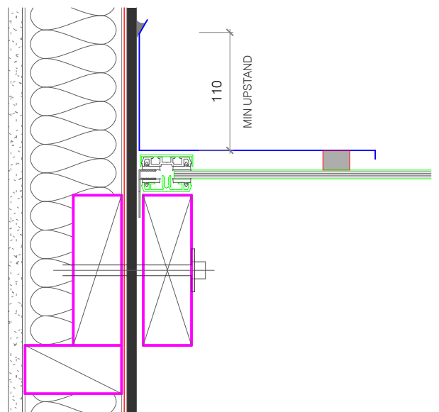
DIRECT FIX DETAIL
