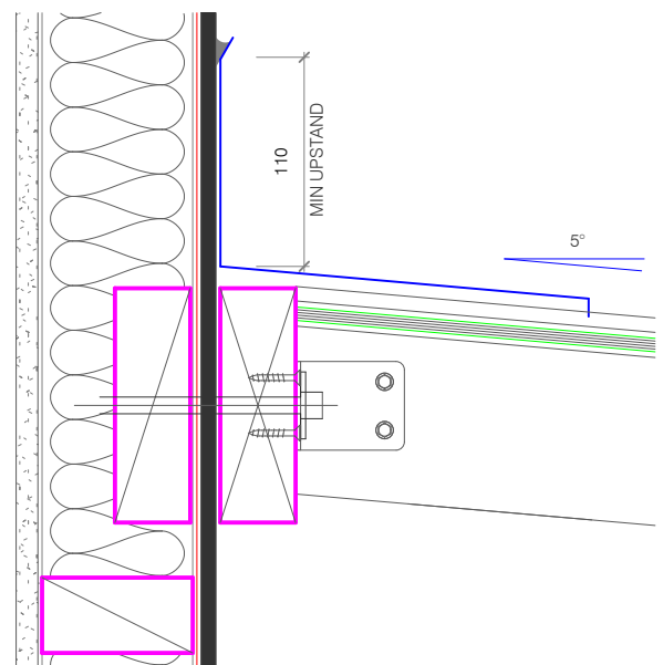
DIRECT FIX DETAIL
