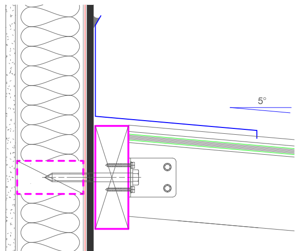
DIRECT FIX DETAIL
